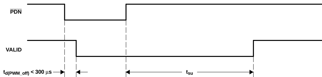
Figure 4-6. Power-Down Timing
