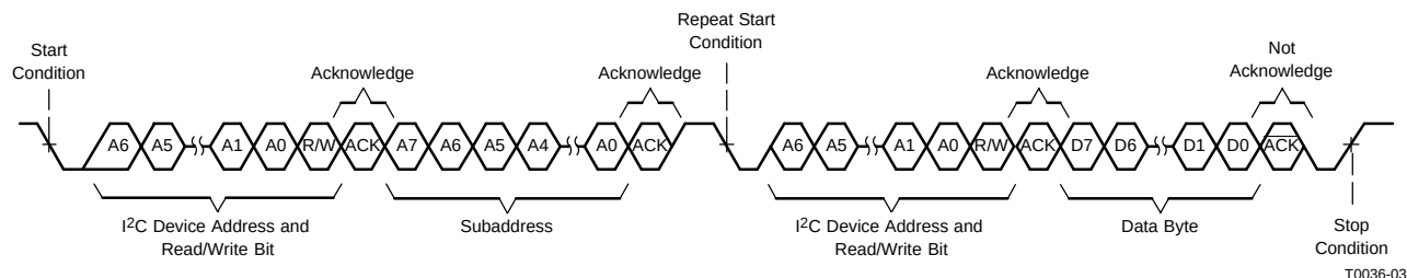
Figure 5-4. Single-Byte Read Transfer
