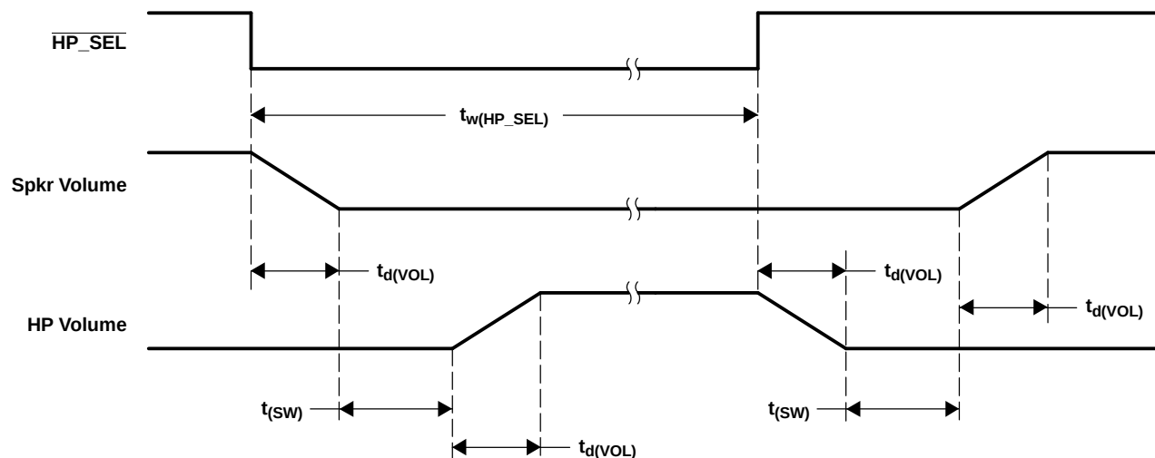
Figure 4-9. \overline{\text{HP\_SEL}} Timing
