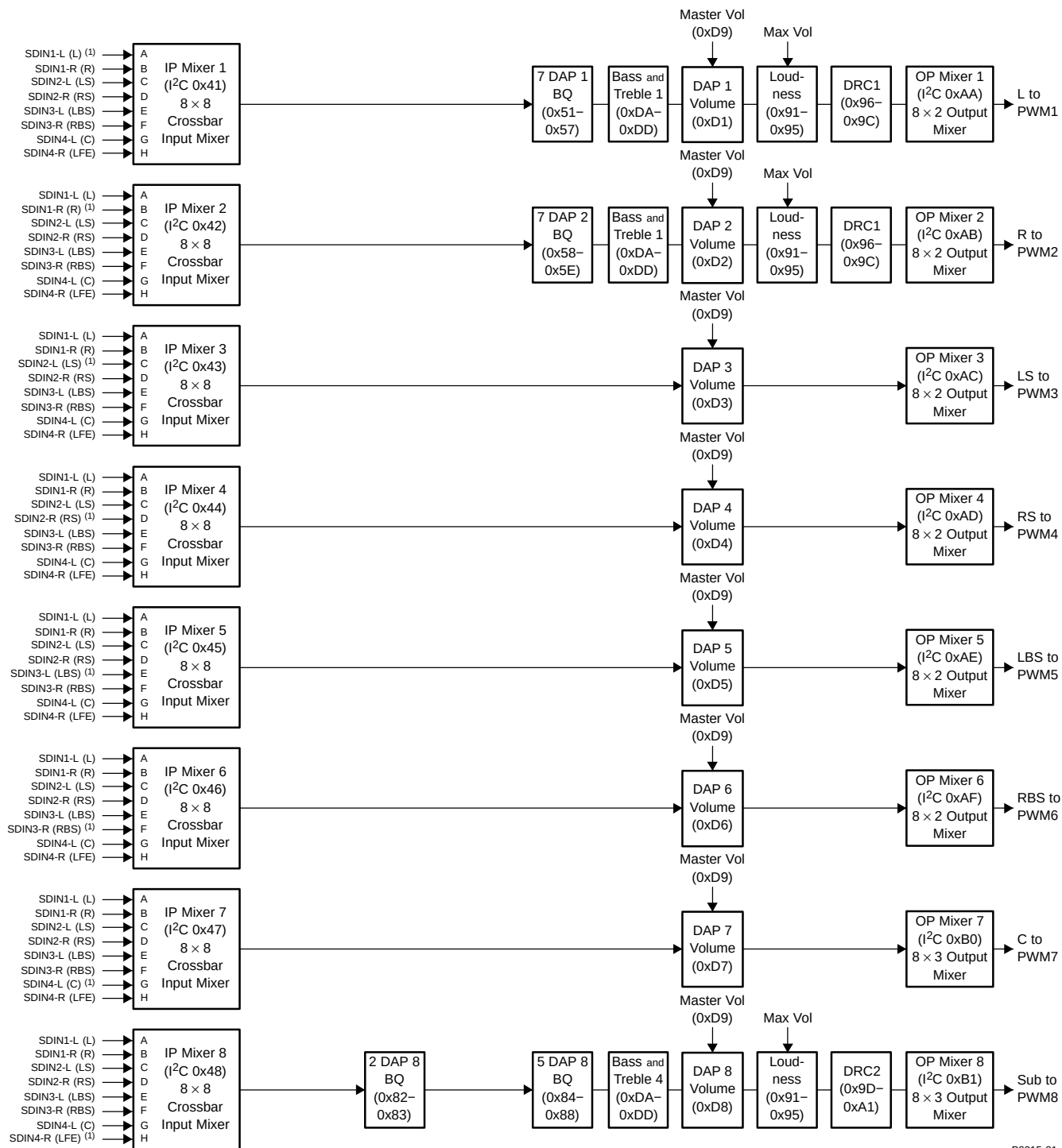
Figure 2-2. TAS5508B Architecture With I 2 C Registers ( f_s = 176.4 kHz or f_s = 192 kHz)
