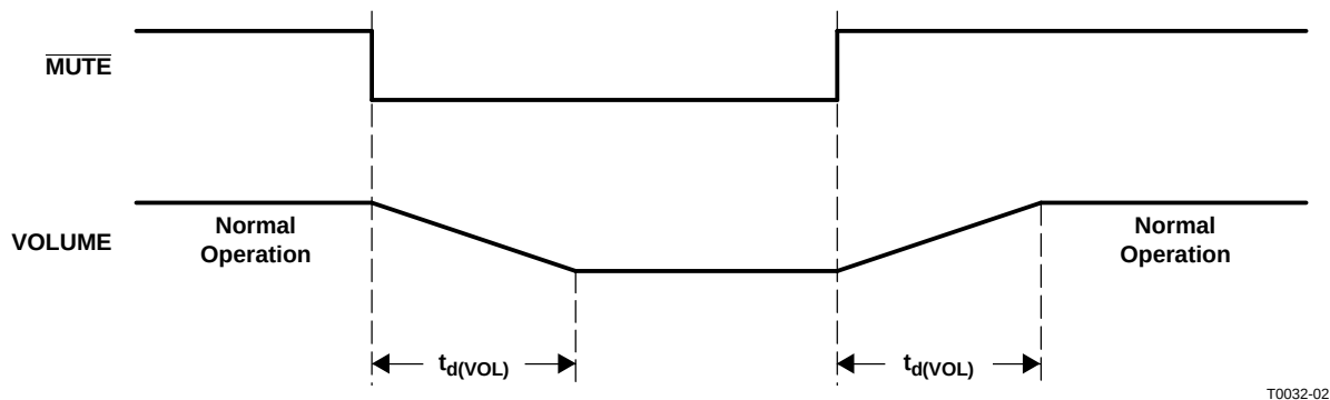
Figure 4-8. Mute Timing
