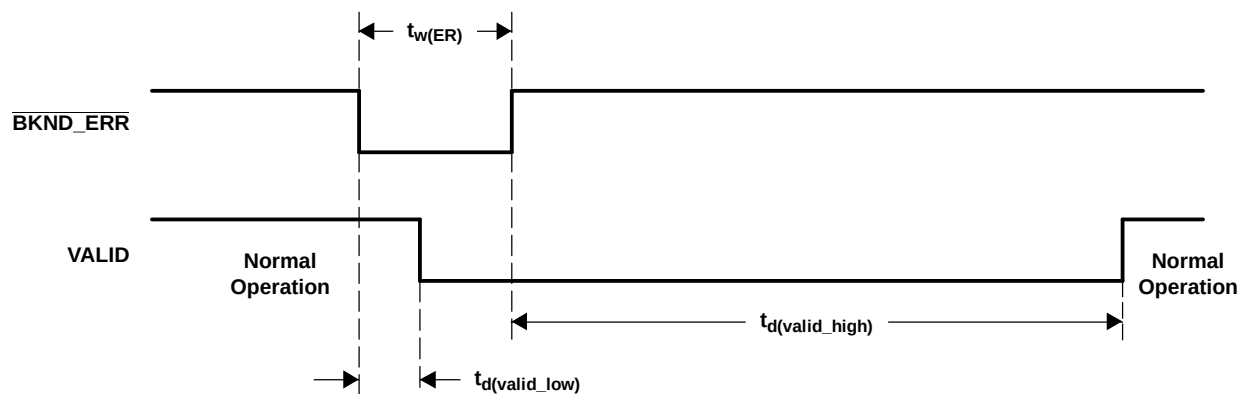
Figure 4-7. Error-Recovery Timing
